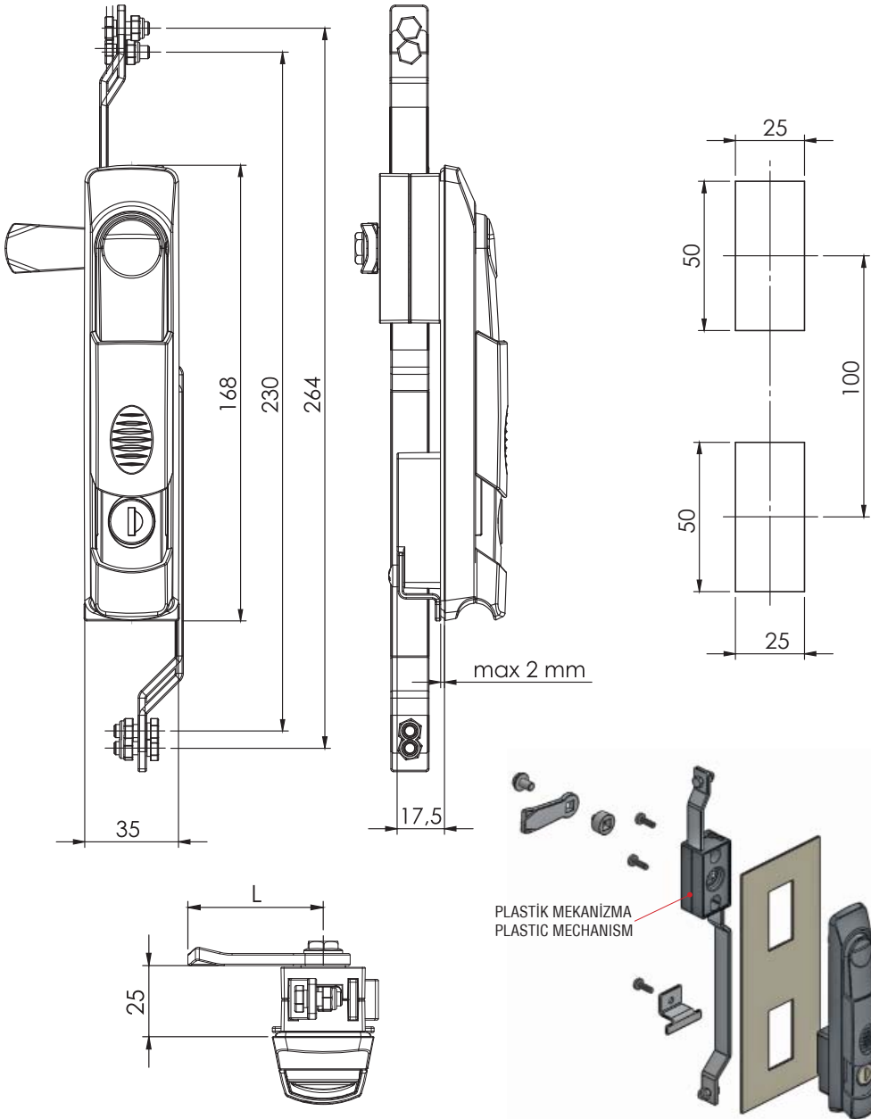
Asma Kilit Padlock Device Selectable
