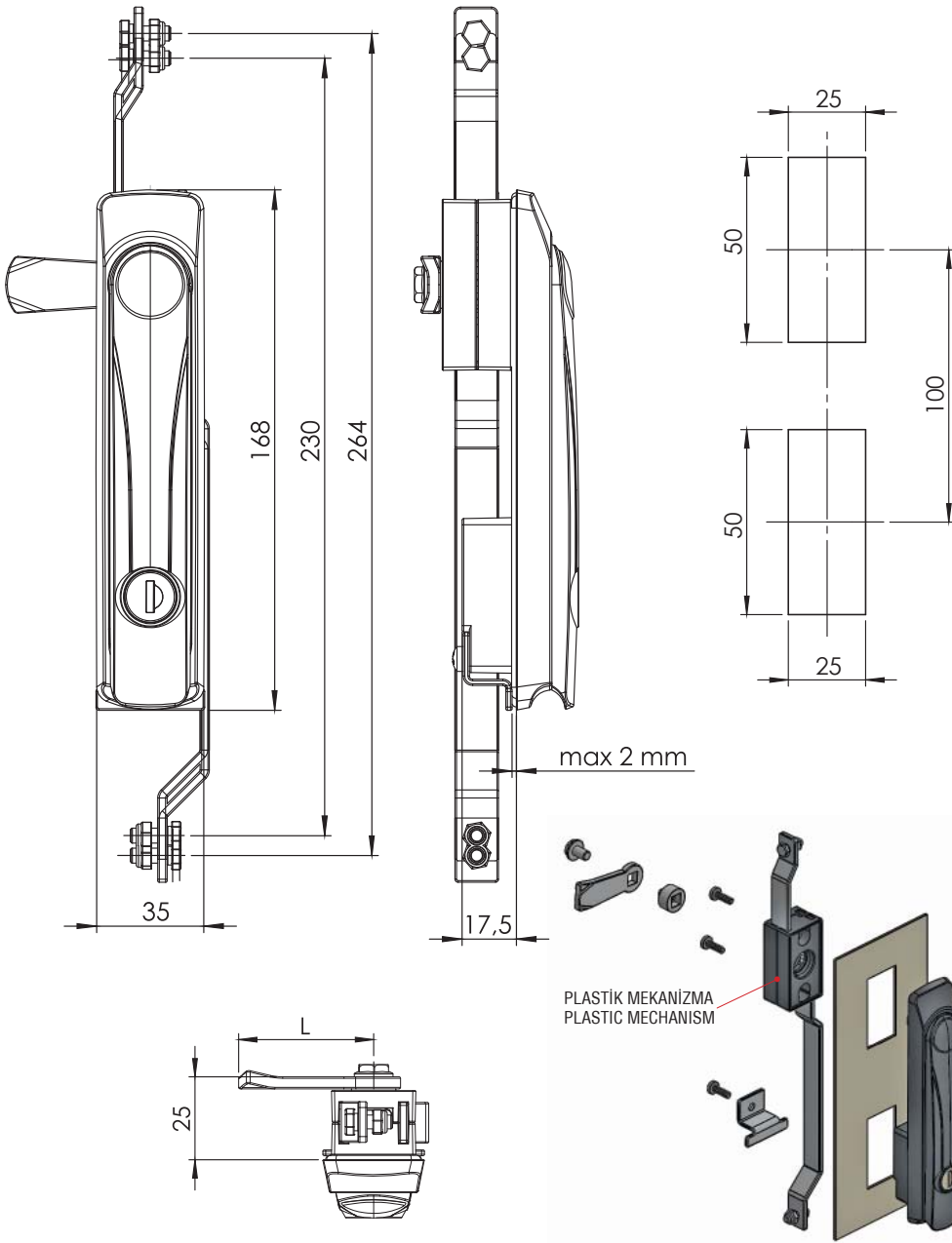
Asma Kilit Padlock Device Selectable
